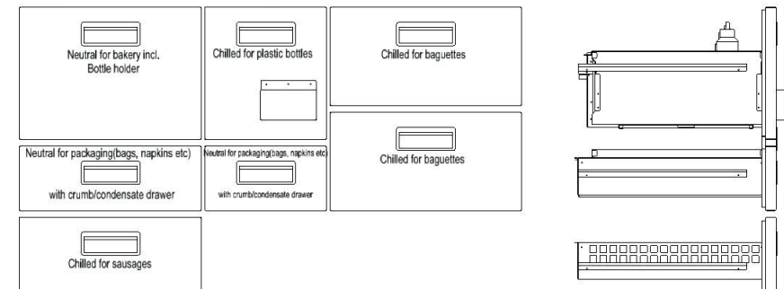
Detail of the inner arrangement of the drawers
