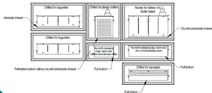
View from the service side on the arrangements of the modules drawers
