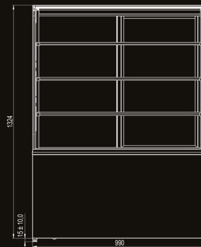
VIRGINIA FREE-STANDING
