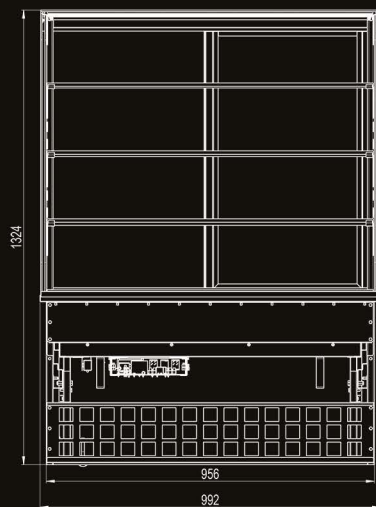
VIRGINIA DROP-IN
